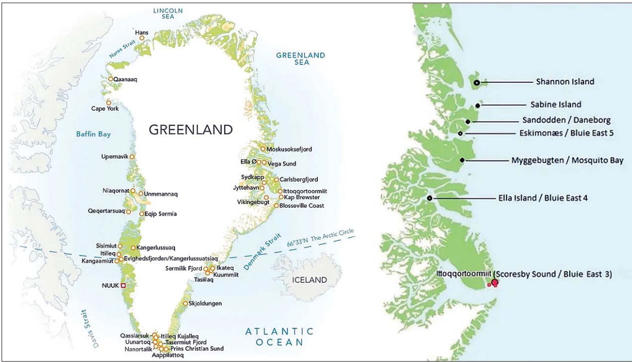
The island of Greenland, showing its central ice sheet, and a map of the North East, showing key locations in this story.
